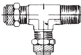
MALE RUN TEE #M71P
